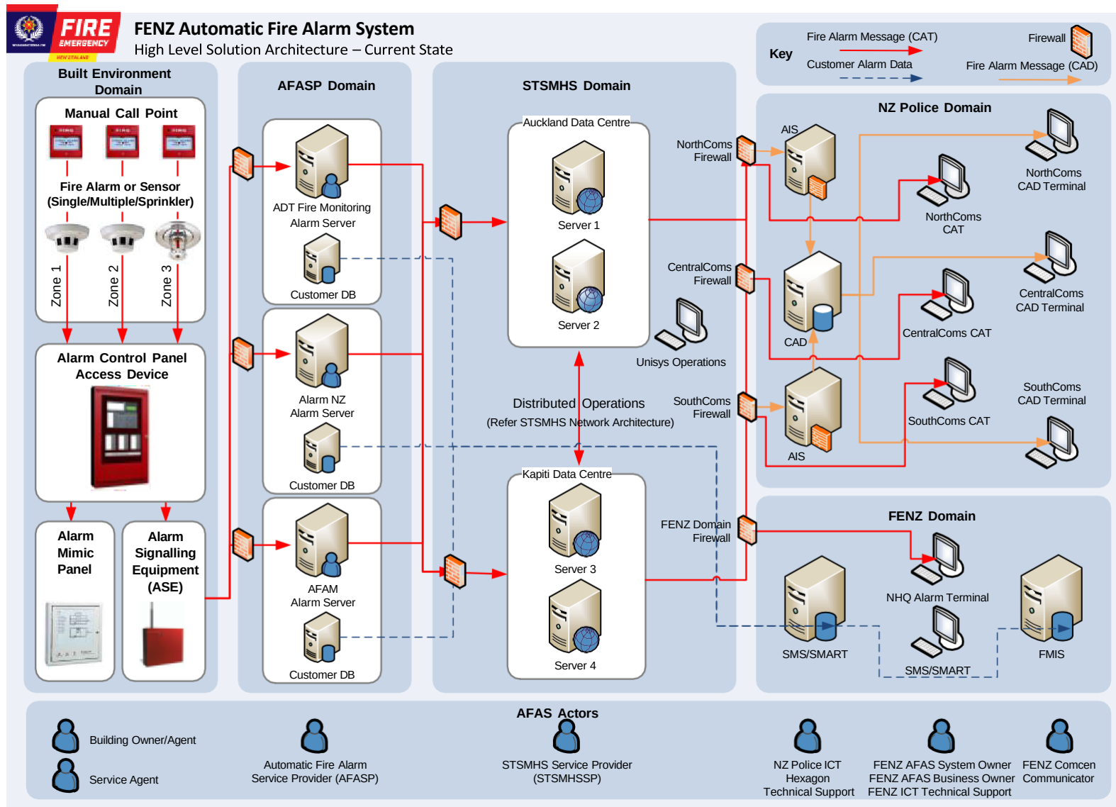
Figure 3. High level solution architecture of the Automatic Fire Alarm System (AFAS)
